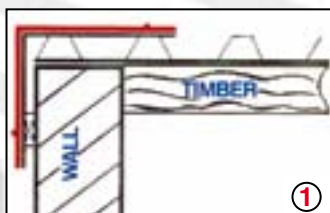
TYPICAL BARGE FLASHING
