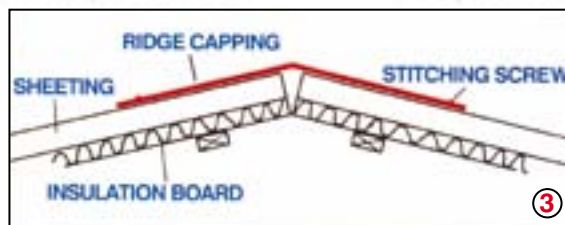
TYPICAL RIDGE FLASHING
