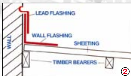
TYPICAL WALL FLASHING
